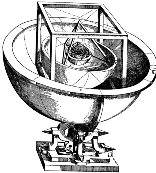
Figure 1 Kepler's model of solar system
